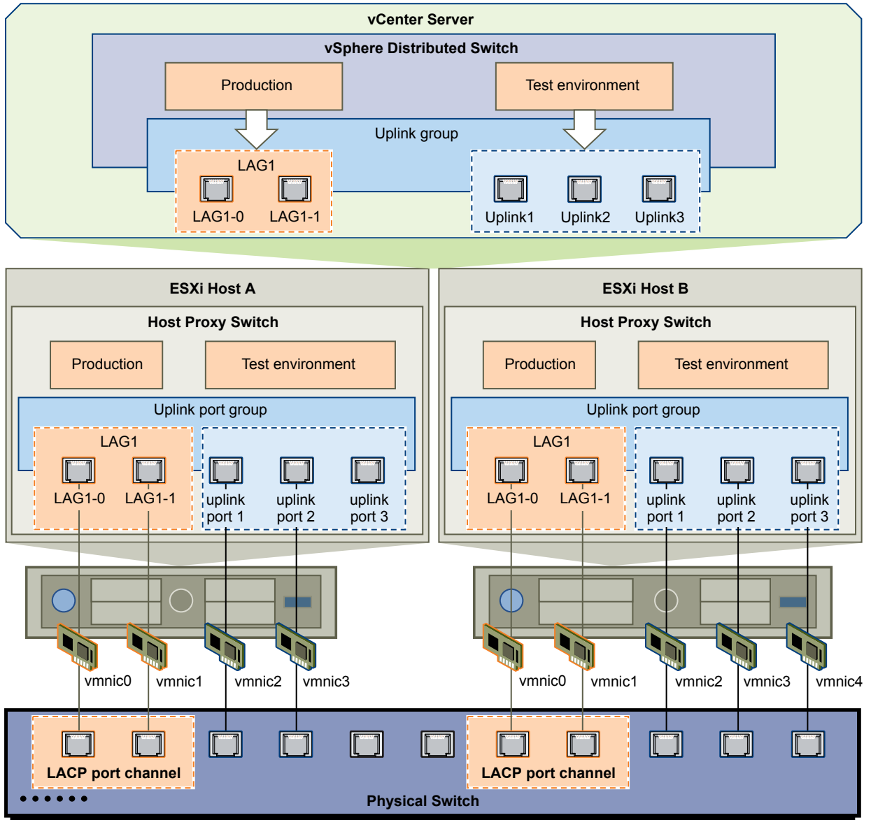
Figure 5-1. Enhanced LACP Support on a vSphere Distributed Switch
