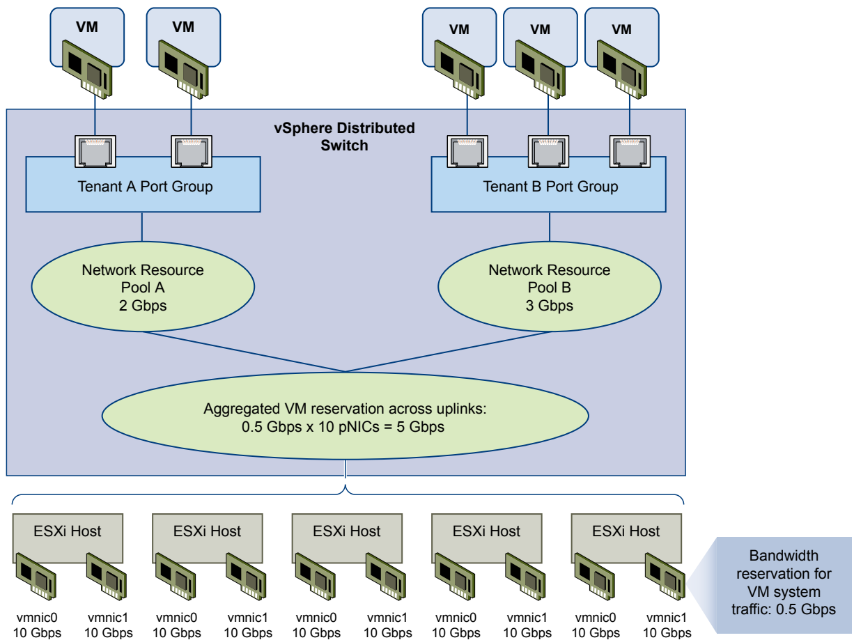
Figure 11-2. Bandwidth Aggregation for Network Resource Pools Across the Uplinks of a vSphere Distributed Switch
