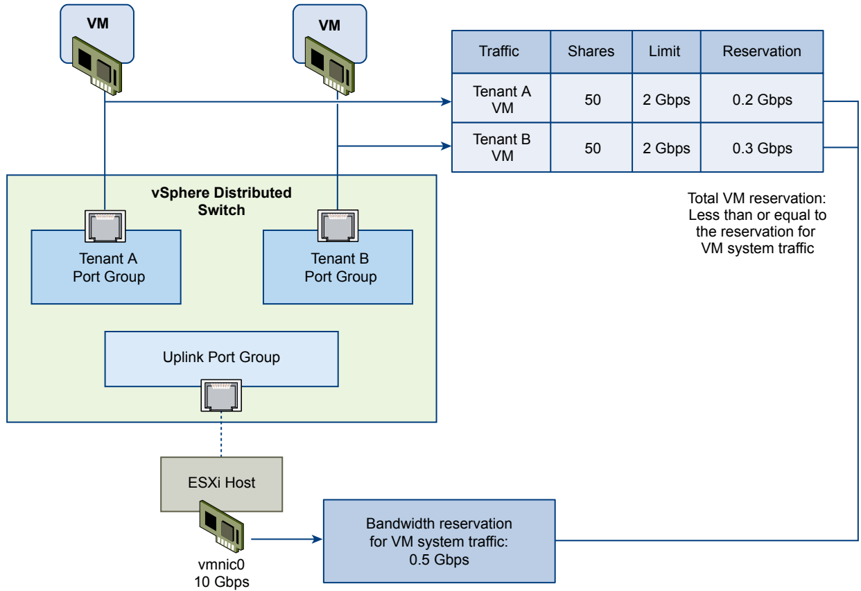
Figure 11-3. Configuration for Bandwidth Allocation for Individual Virtual Machines
